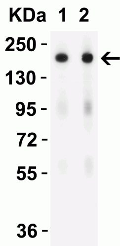
Figure 2 Overexpression Validation in Spike Transfected 293 Cells
